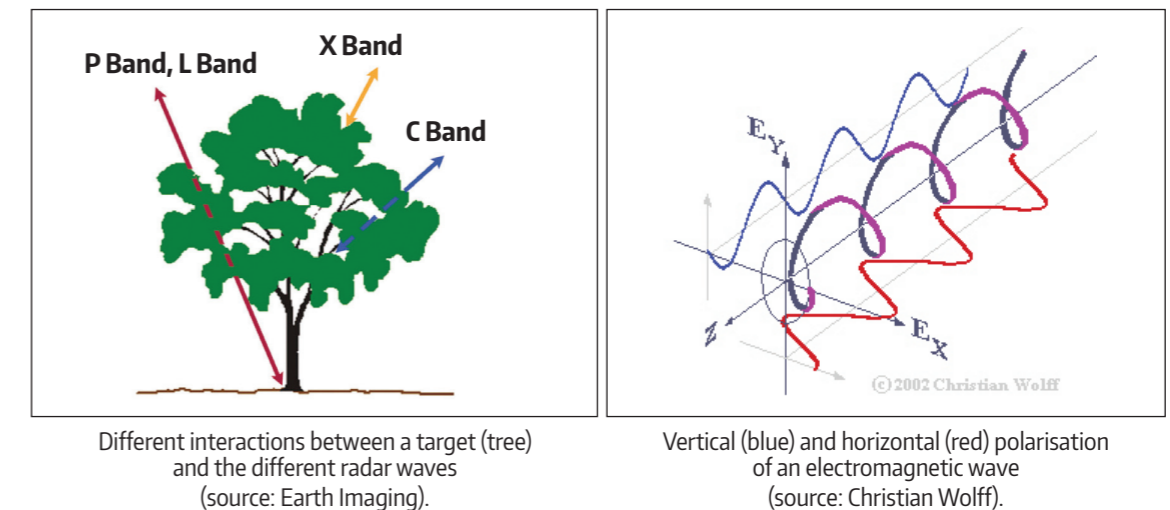
Figure 59: Interaction of the radar signal with the targets and its signal polarisation.
