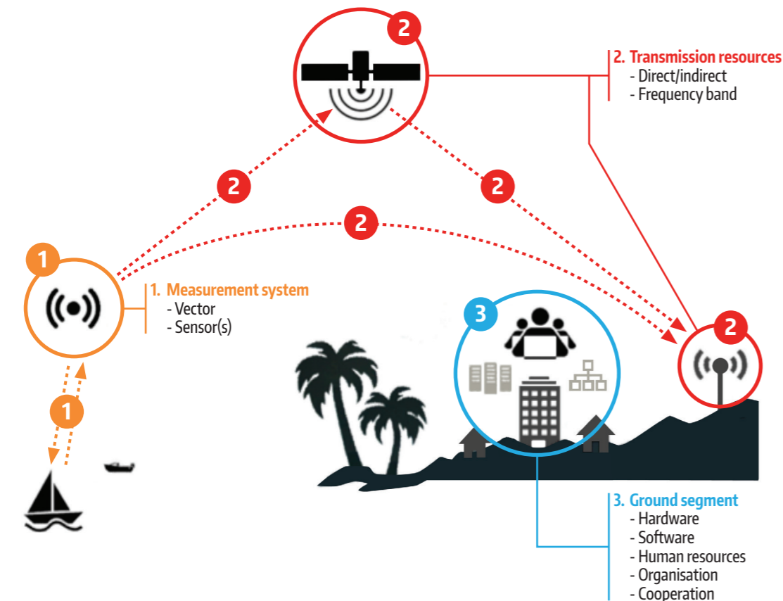
Figure 41: Standard architecture for monitoring and tracking technology.
