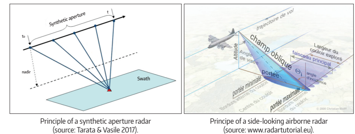
Figure 58: Principles of radar sensors.
