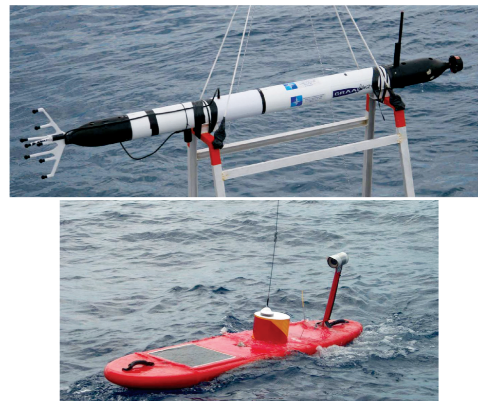
Figure 78: Top, eFolaga autonomous underwater vehicle (source: Maguer et al. 2013), bottom, Liquid Robotics's Wave Glider unmanned surface vehicle (source: Manley 2008).
